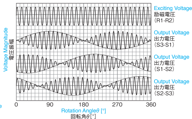
Fig.2 Output Voltage of Control Synchro (in case of CX & BCX)
